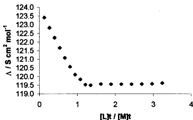
Figure 2. Plot of \Lambda vs. [L]t/[M]t for \text{AgNO}_3 and 18C6 in 1% TX 100.
