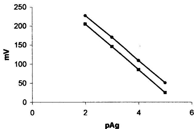
Figure 1. Plot of emf vs. silver-ion concentration in: ●, aqueous medium; ◆, 1% TritonX 100.
