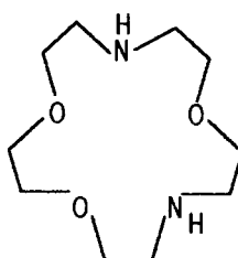
diaza-15C5
