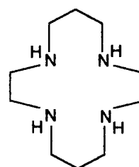
cyclam
